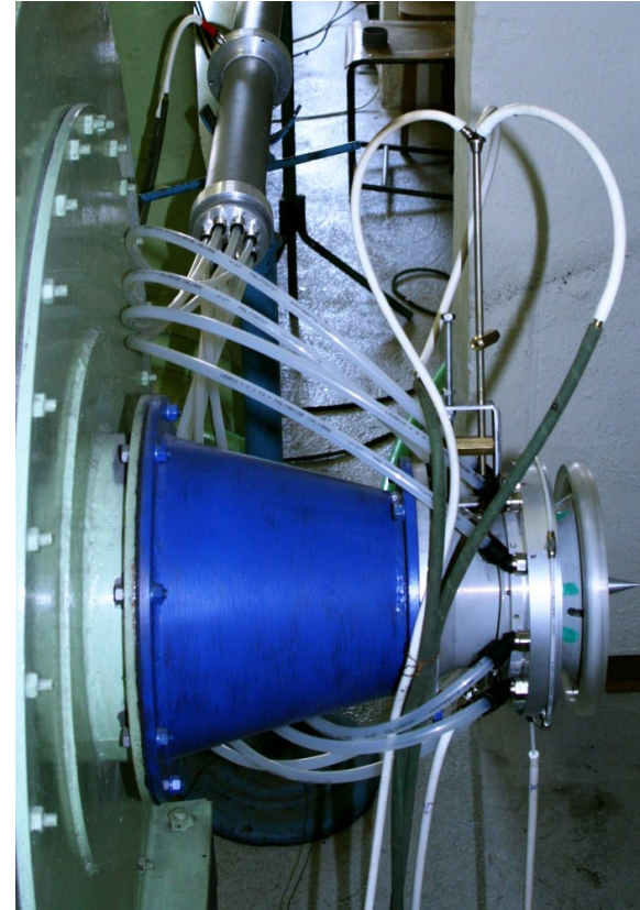
Measurement at the Inlet of Centrifugal Compressor
