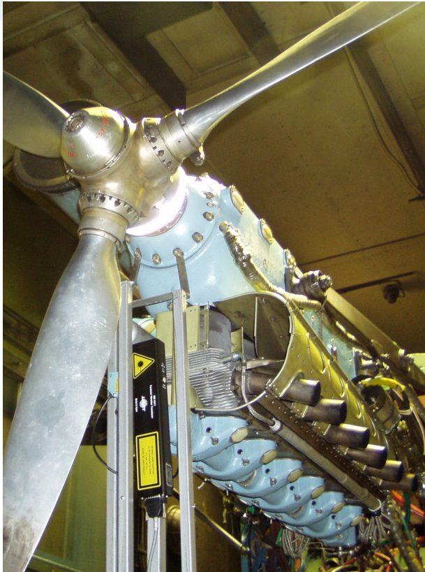
Torsion vibrations of Aircraft Engine with Propeller
